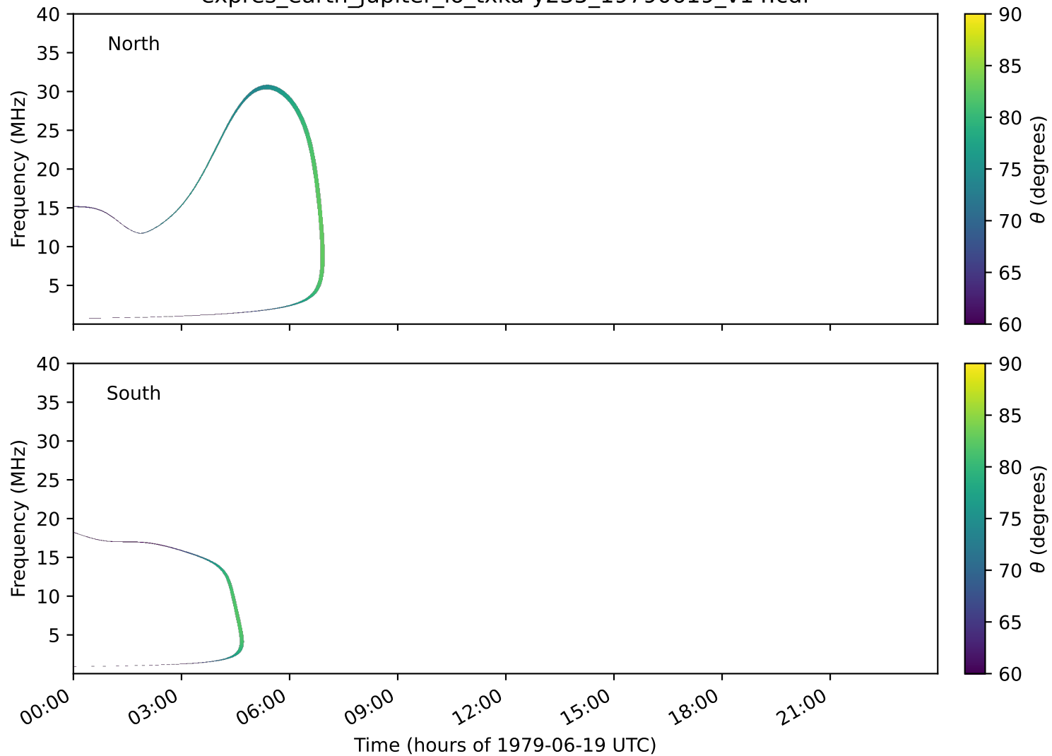
expres_earth_jupiter_io_txka-y235_19790619_v14.cdf
