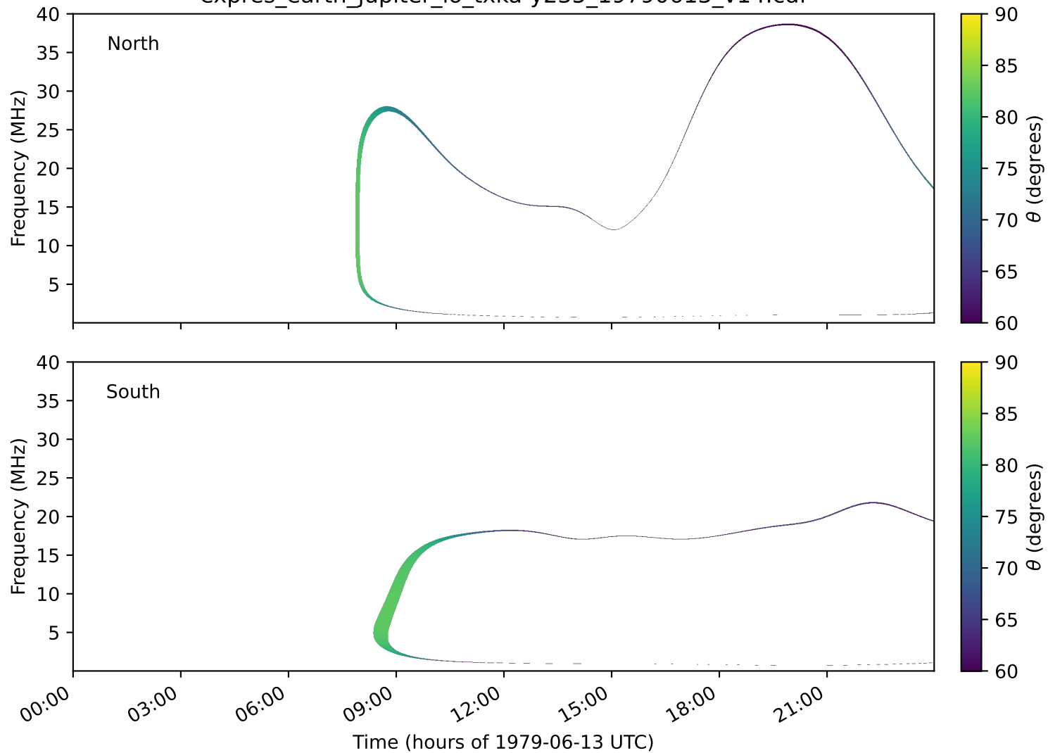
expres_earth_jupiter_io_txka-y235_19790613_v14.cdf
