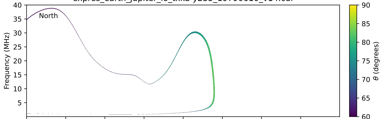
expres_earth_jupiter_io_txka-y235_19790610_v14.cdf
