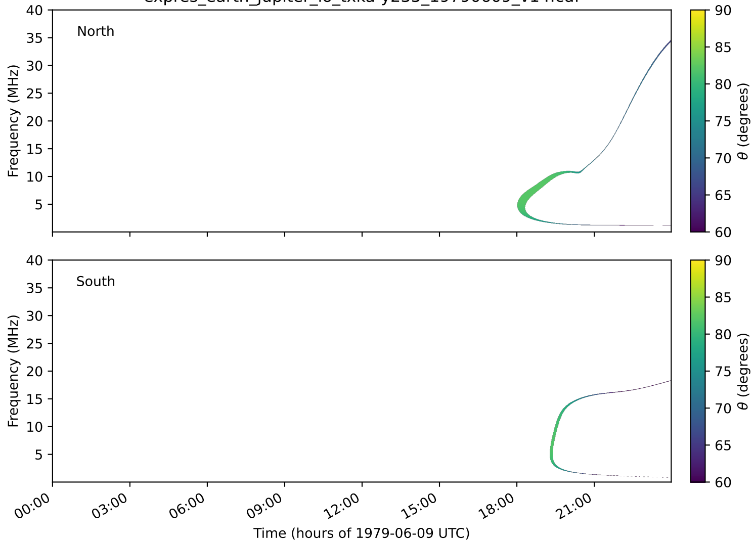
expres_earth_jupiter_io_txka-y235_19790609_v14.cdf
