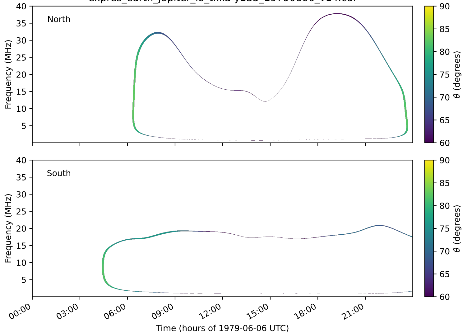
expres_earth_jupiter_io_txka-y235_19790606_v14.cdf
