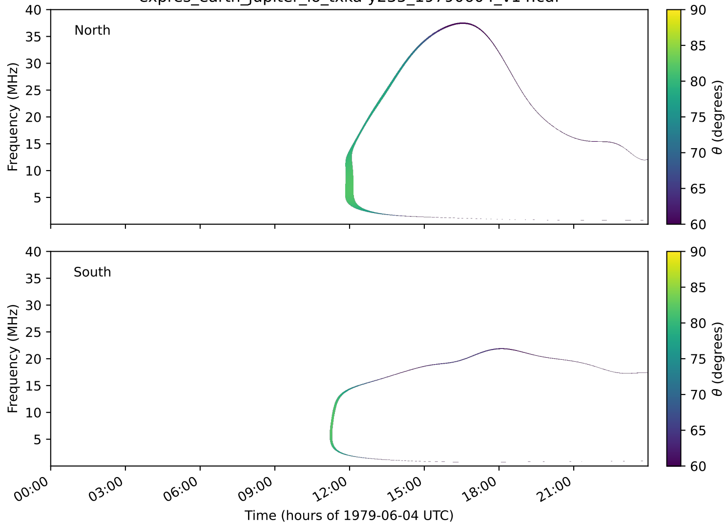
expres_earth_jupiter_io_txka-y235_19790604_v14.cdf
