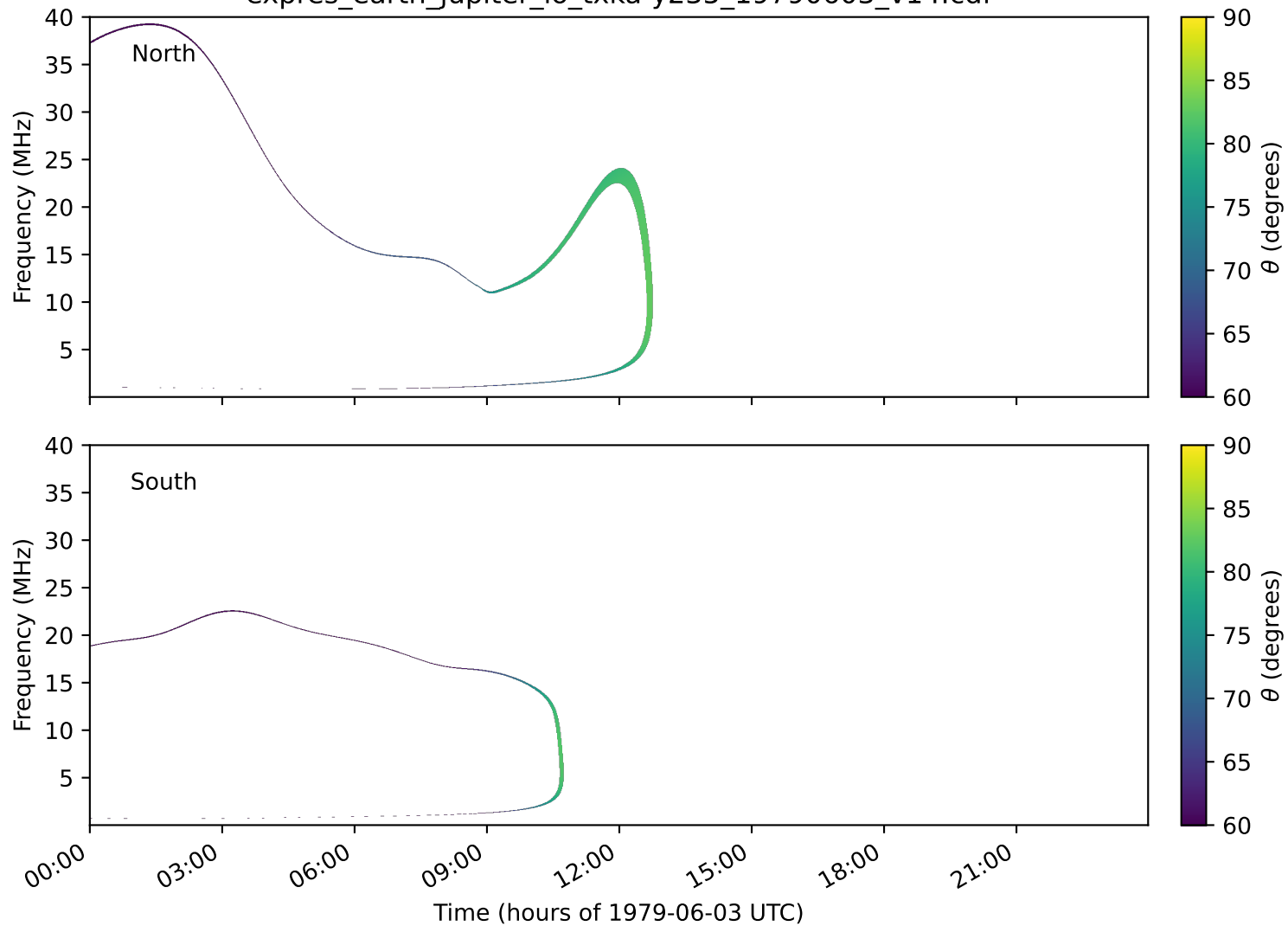
expres_earth_jupiter_io_txka-y235_19790603_v14.cdf
