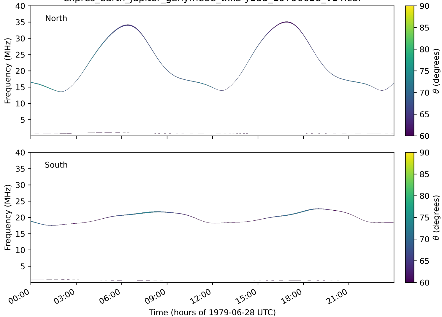
expres_earth_jupiter_ganymede_txka-y235_19790628_v14.cdf
