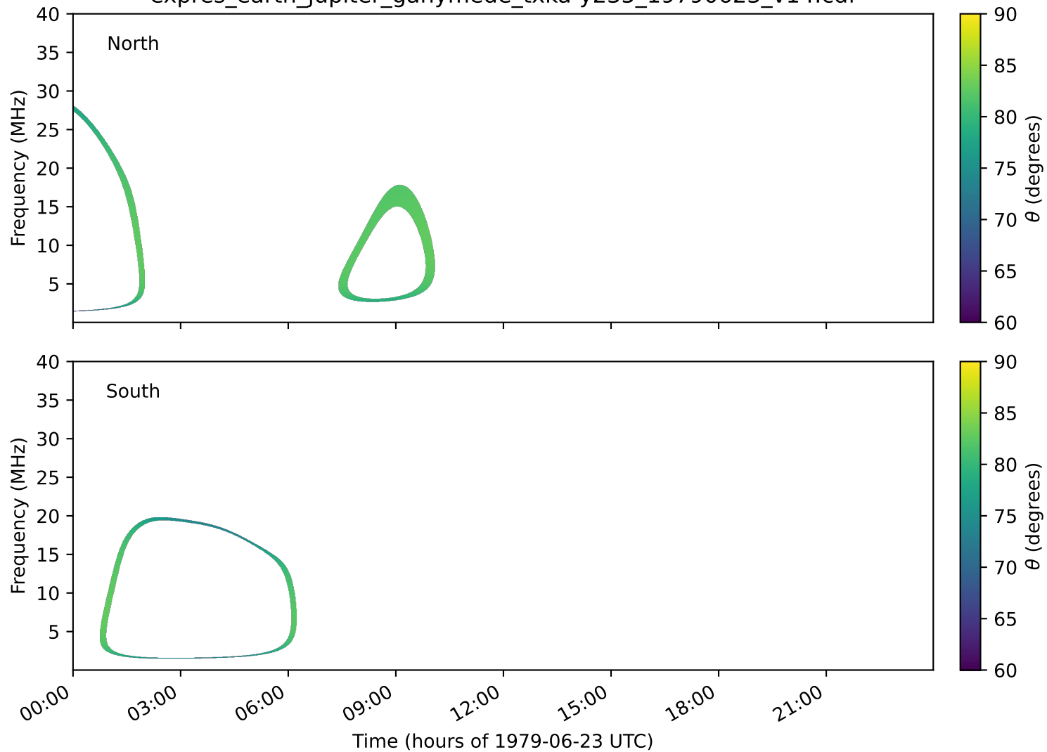
expres_earth_jupiter_ganymede_txka-y235_19790623_v14.cdf
