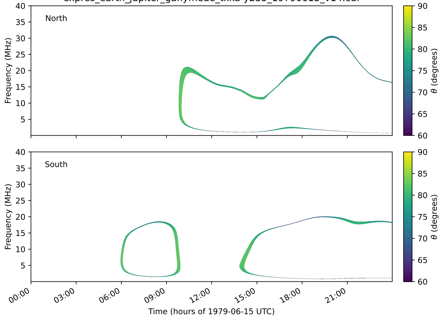
expres_earth_jupiter_ganymede_txka-y235_19790615_v14.cdf
