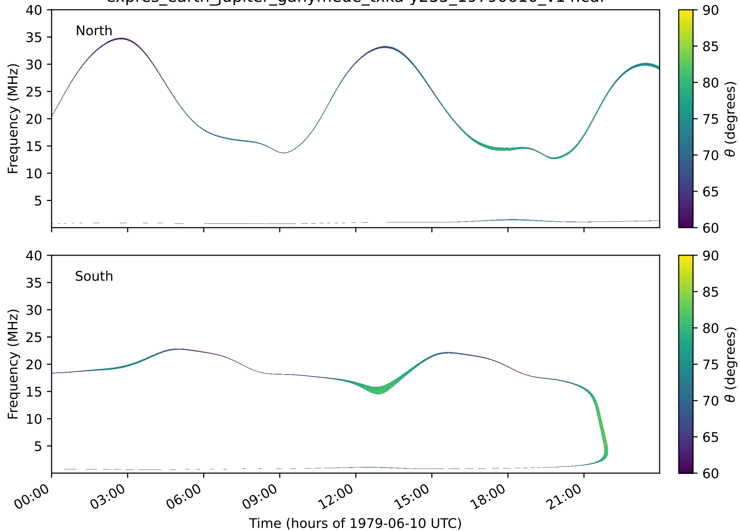
expres_earth_jupiter_ganymede_txka-y235_19790610_v14.cdf
