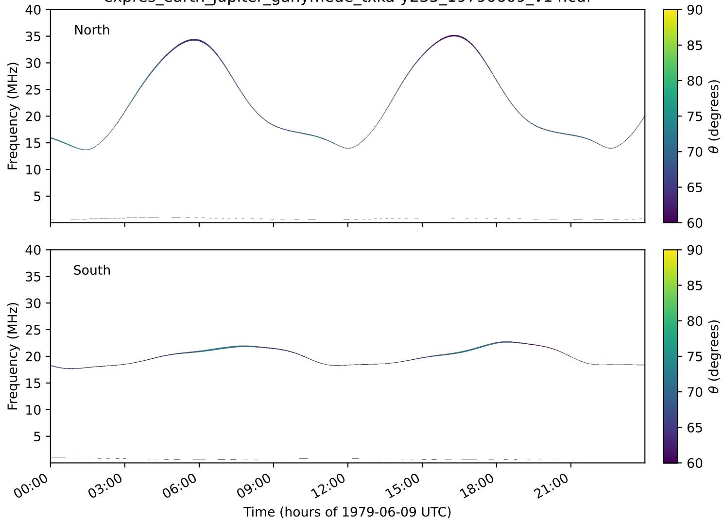
expres_earth_jupiter_ganymede_txka-y235_19790609_v14.cdf
