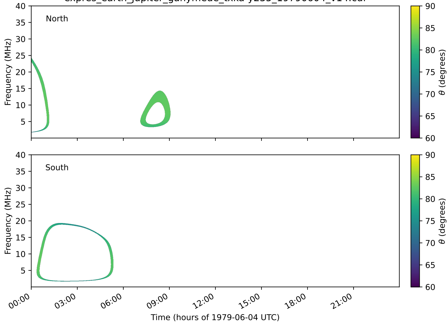
expres_earth_jupiter_ganymede_txka-y235_19790604_v14.cdf
