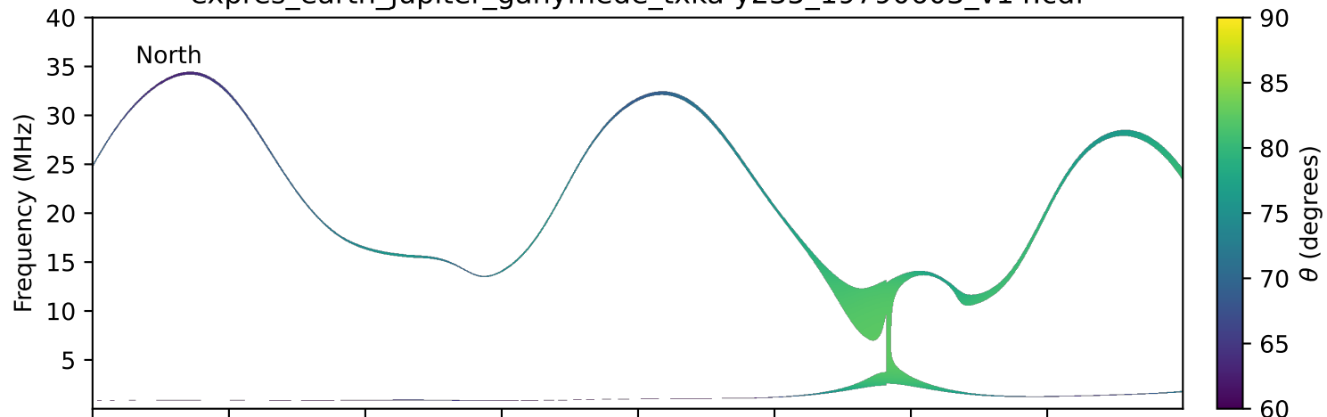
expres_earth_jupiter_ganymede_txka-y235_19790603_v14.cdf
