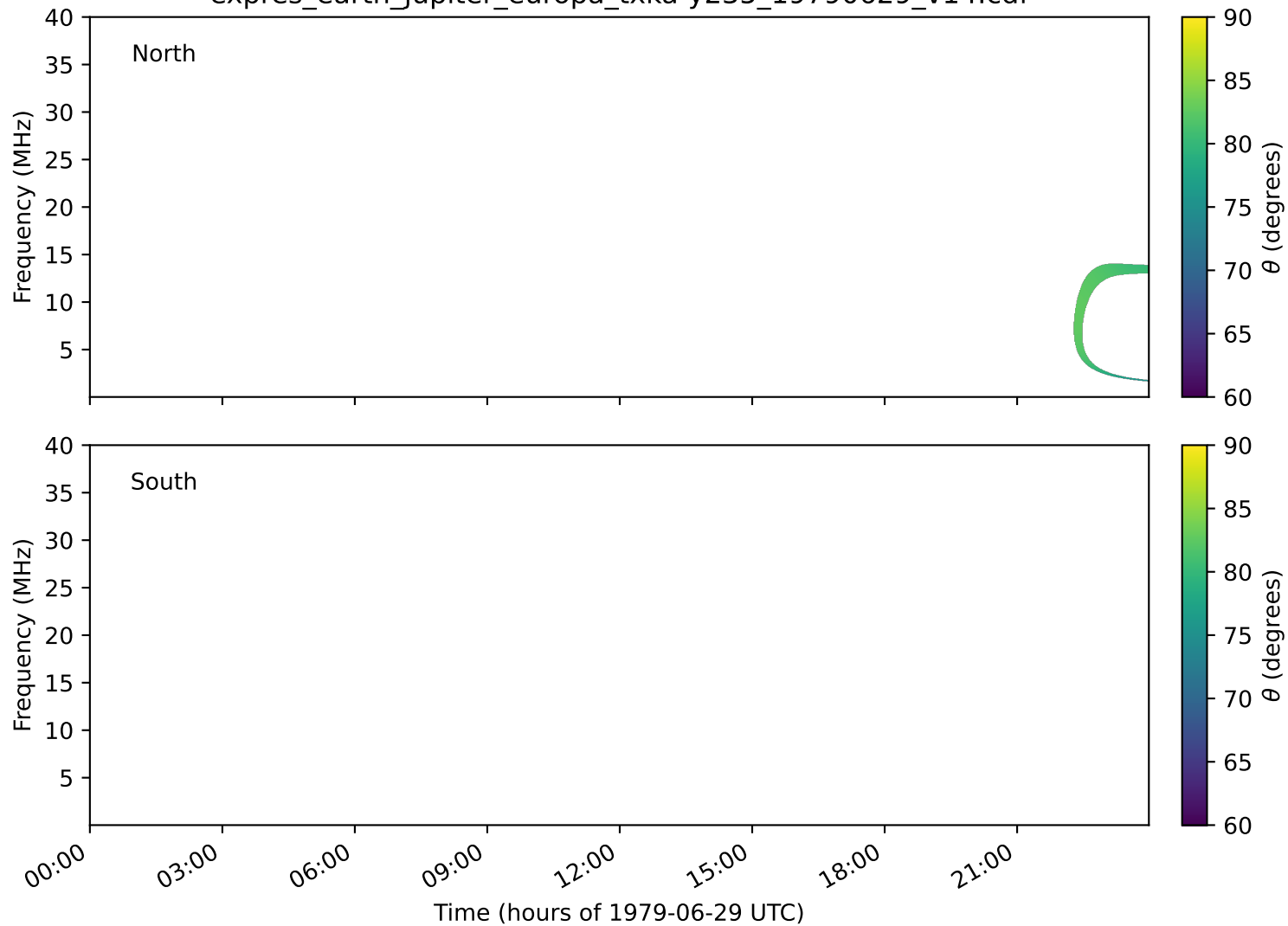
expres_earth_jupiter_europa_txka-y235_19790629_v14.cdf
