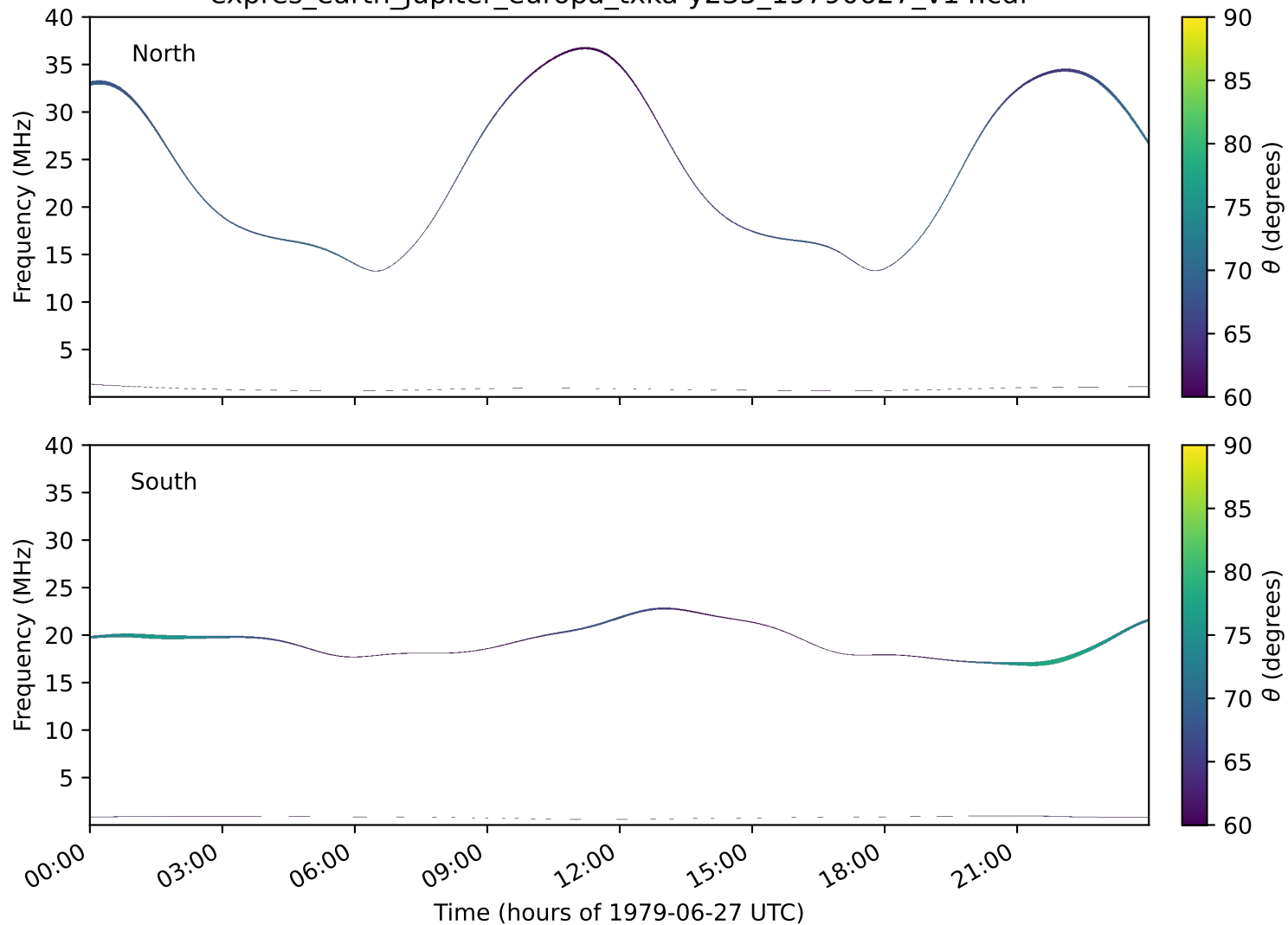
expres_earth_jupiter_europa_txka-y235_19790627_v14.cdf
