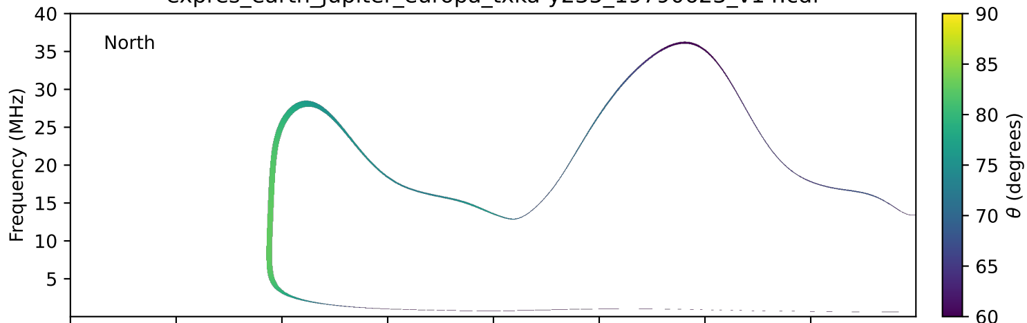
expres_earth_jupiter_europa_txka-y235_19790623_v14.cdf
