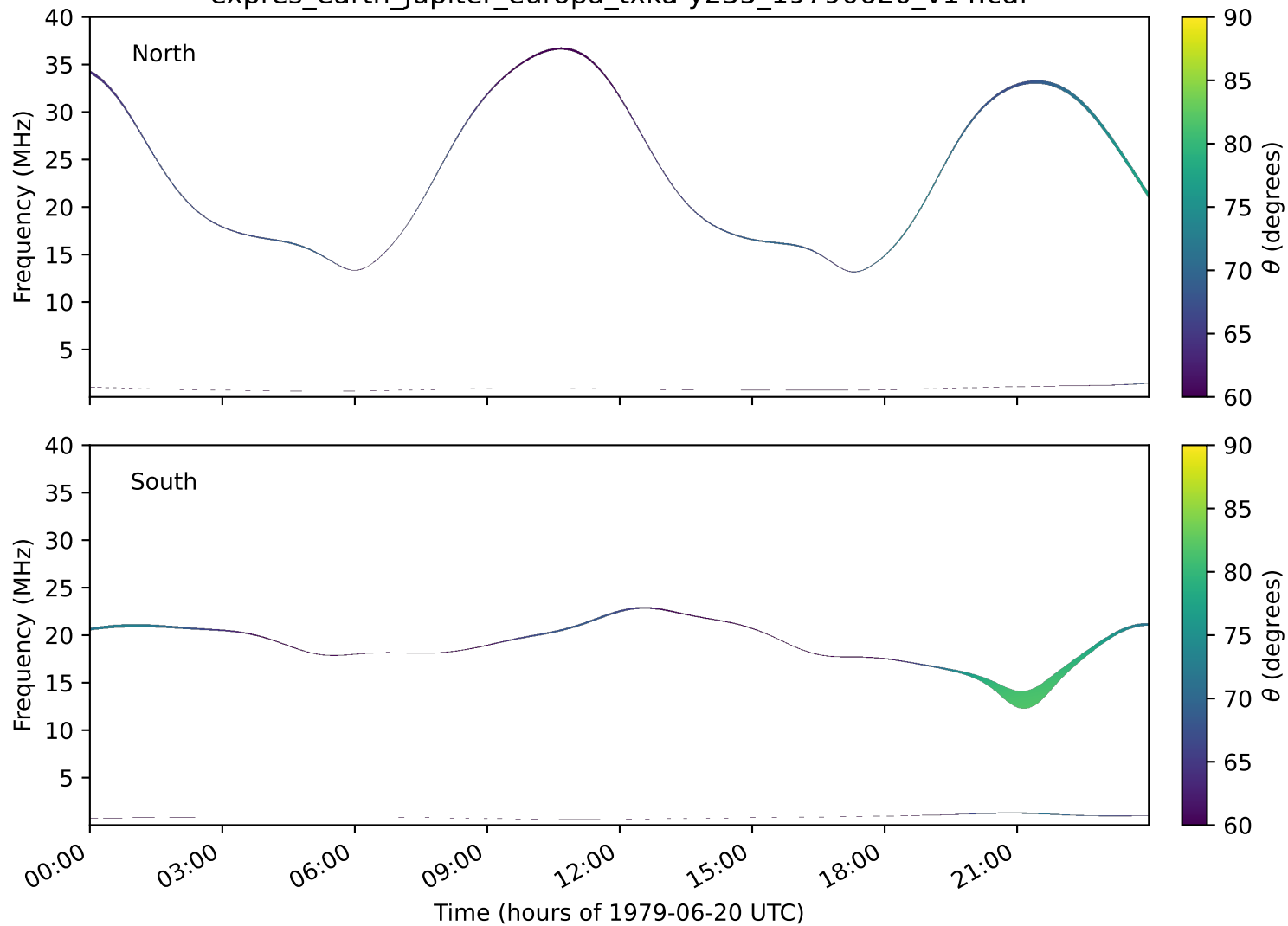
expres_earth_jupiter_europa_txka-y235_19790620_v14.cdf
