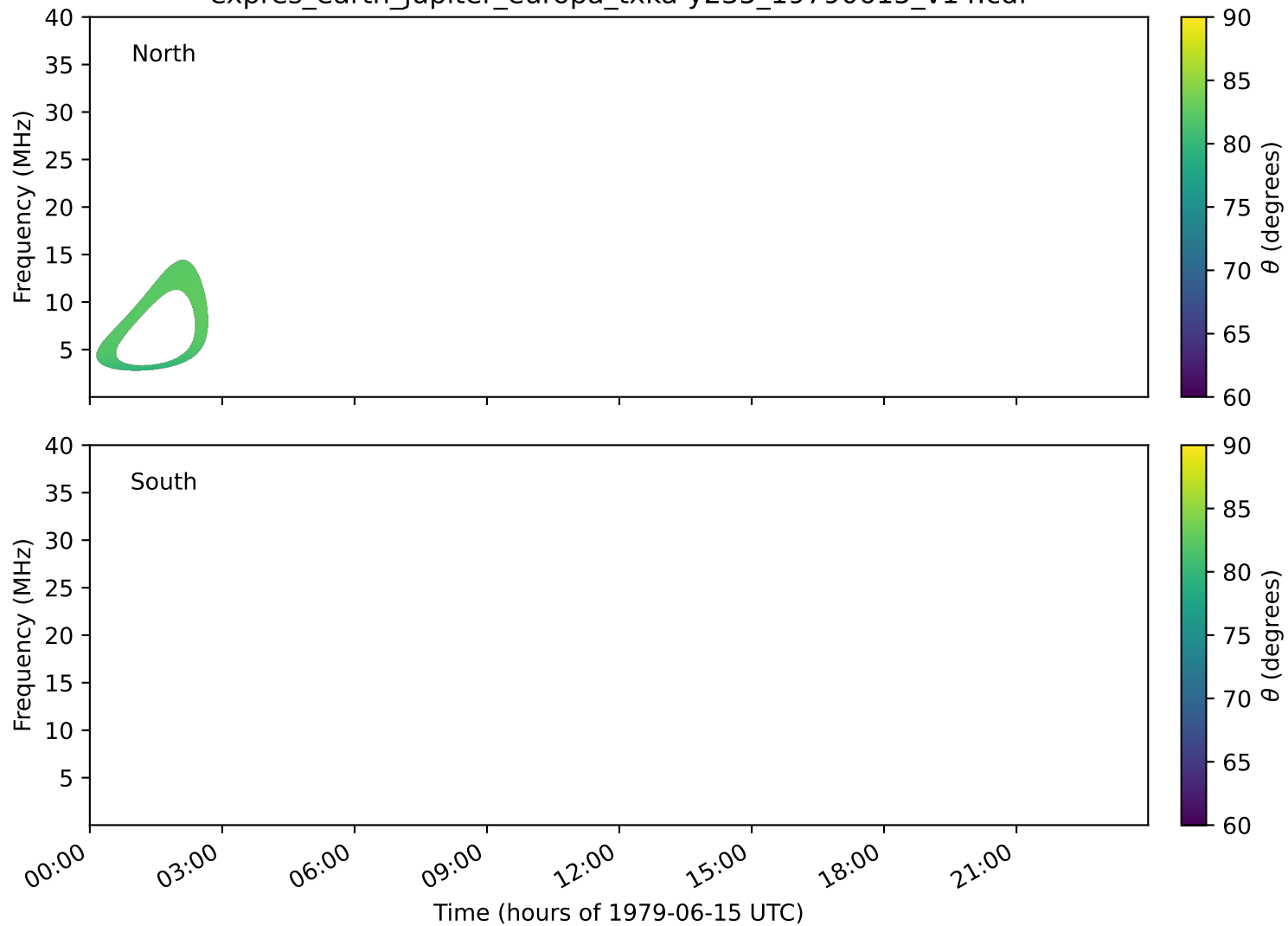
expres_earth_jupiter_europa_txka-y235_19790615_v14.cdf
