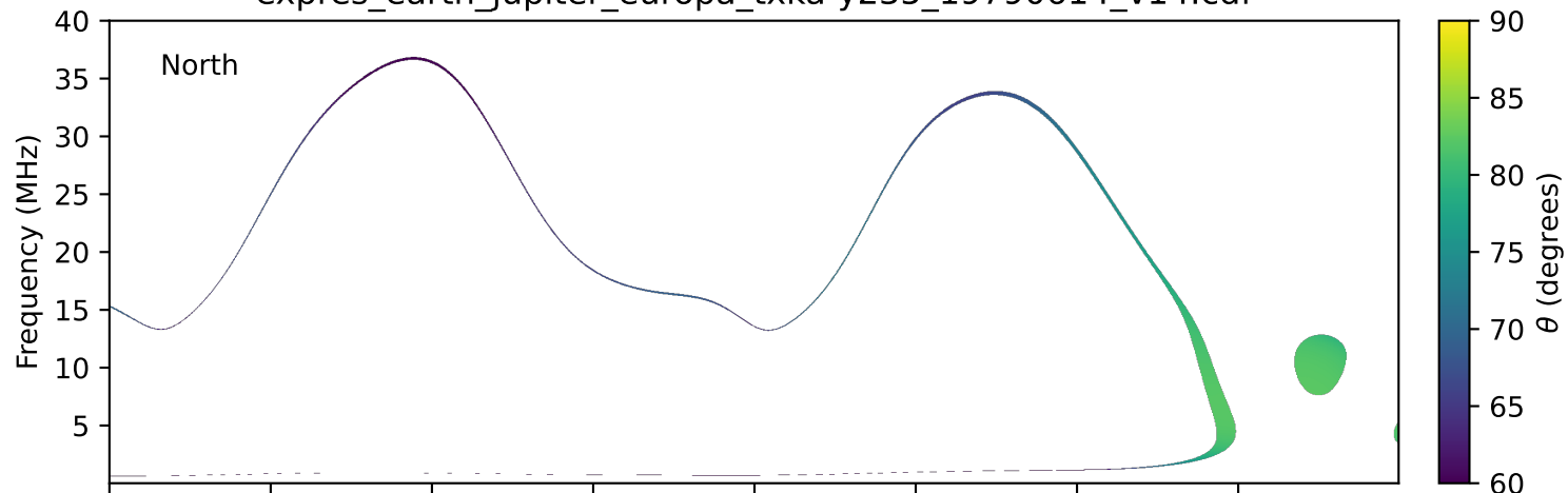
expres_earth_jupiter_europa_txka-y235_19790614_v14.cdf
