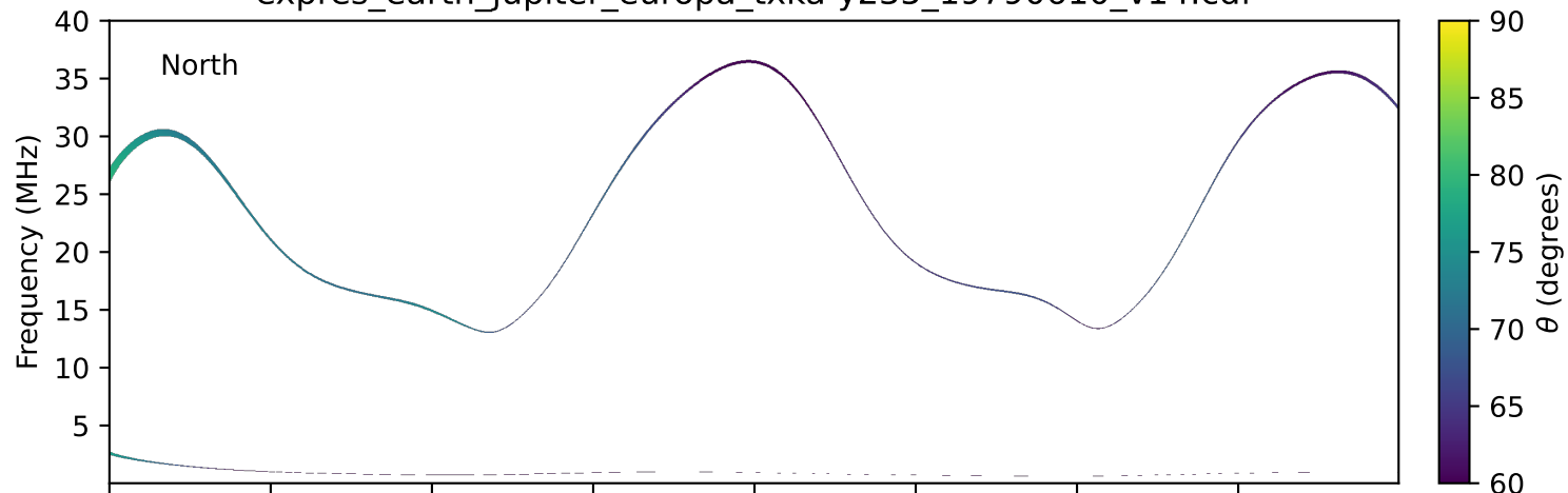
expres_earth_jupiter_europa_txka-y235_19790610_v14.cdf
