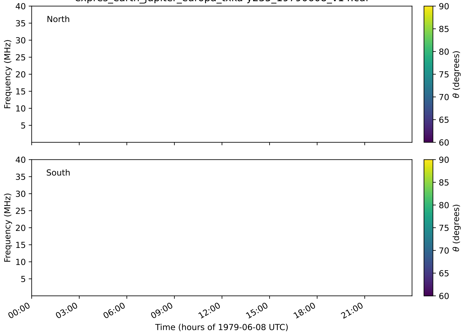
expres_earth_jupiter_europa_txka-y235_19790608_v14.cdf
