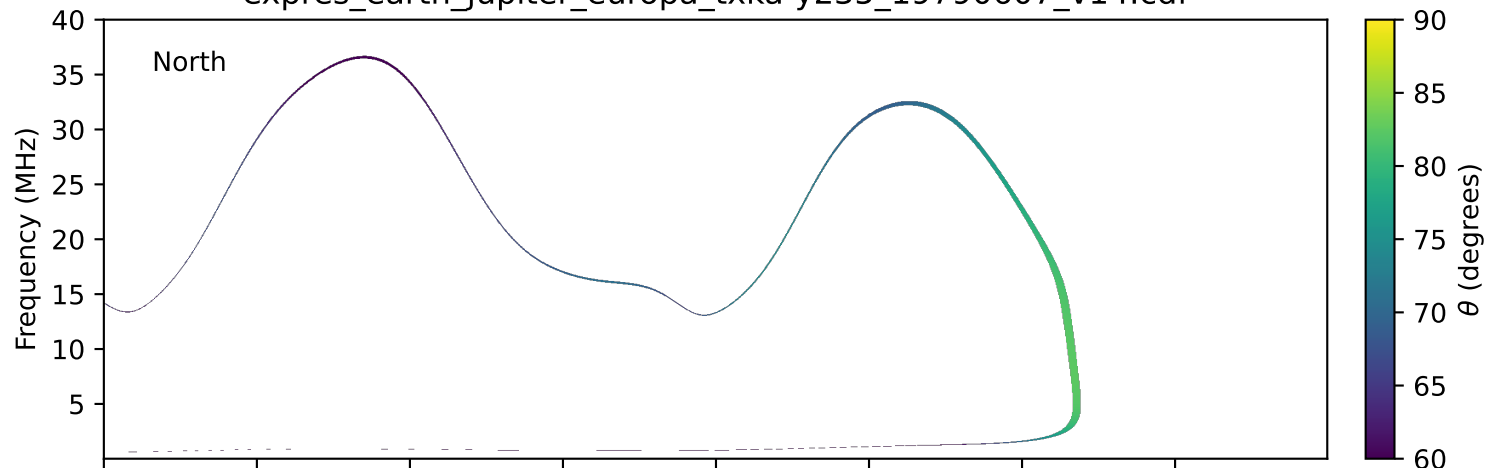
expres_earth_jupiter_europa_txka-y235_19790607_v14.cdf
