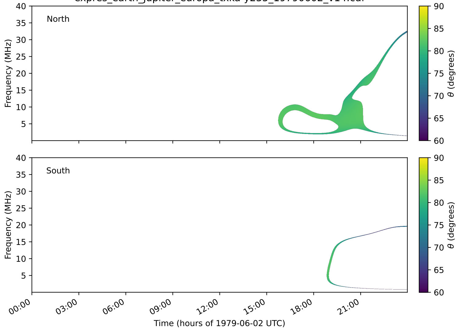
expres_earth_jupiter_europa_txka-y235_19790602_v14.cdf
