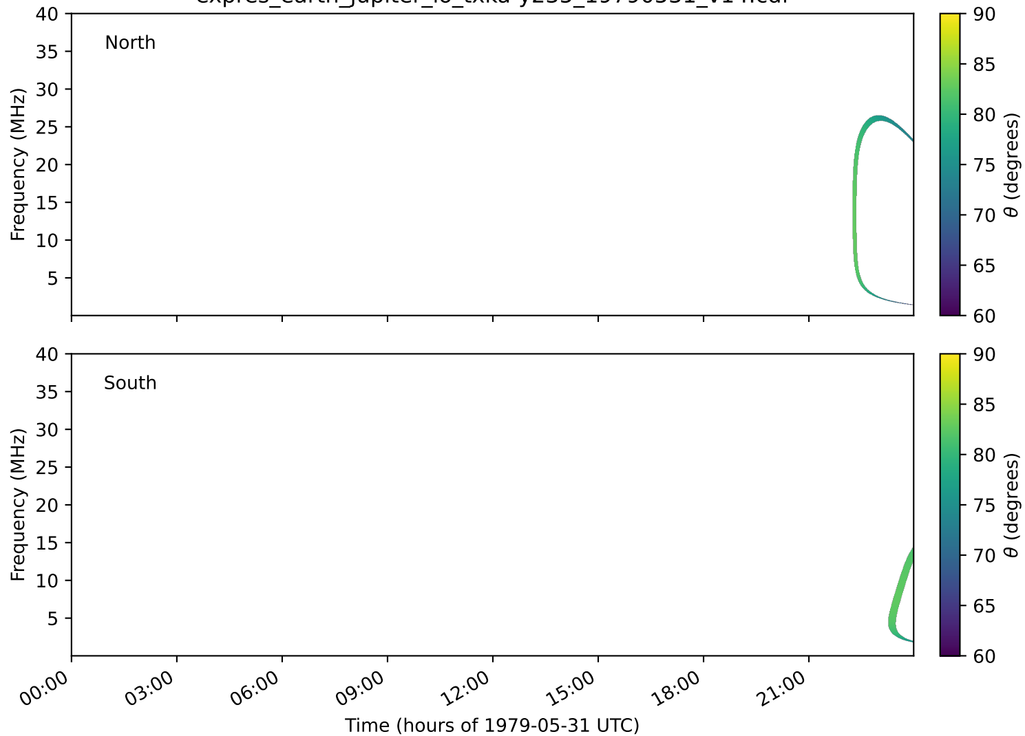
expres_earth_jupiter_io_txka-y235_19790531_v14.cdf
