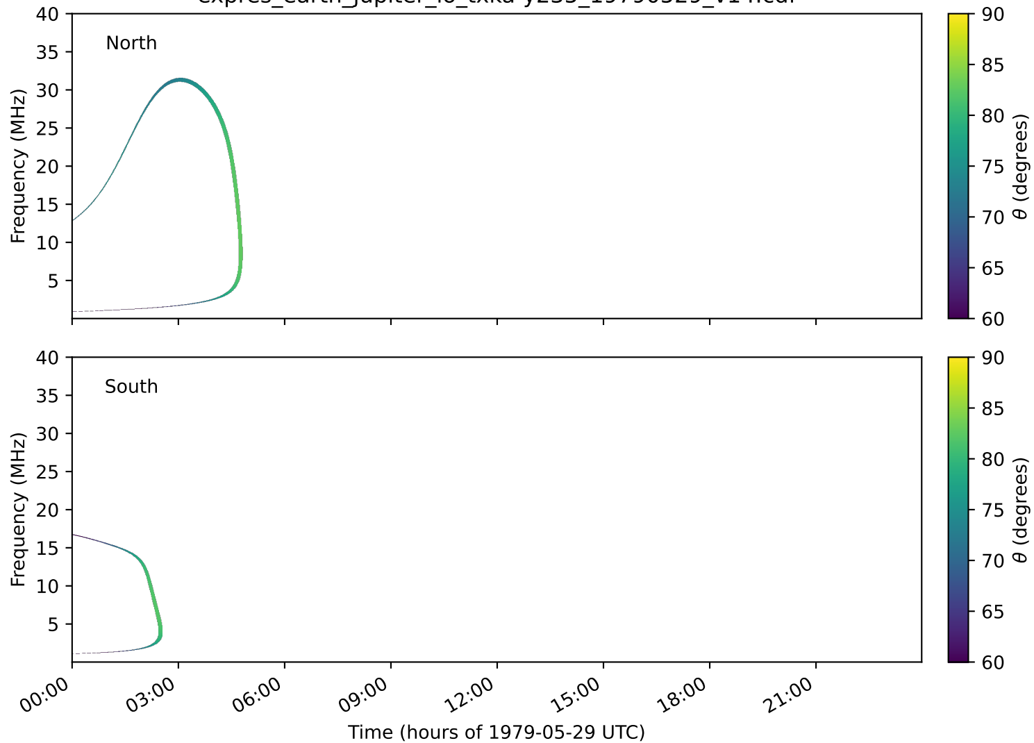
expres_earth_jupiter_io_txka-y235_19790529_v14.cdf
