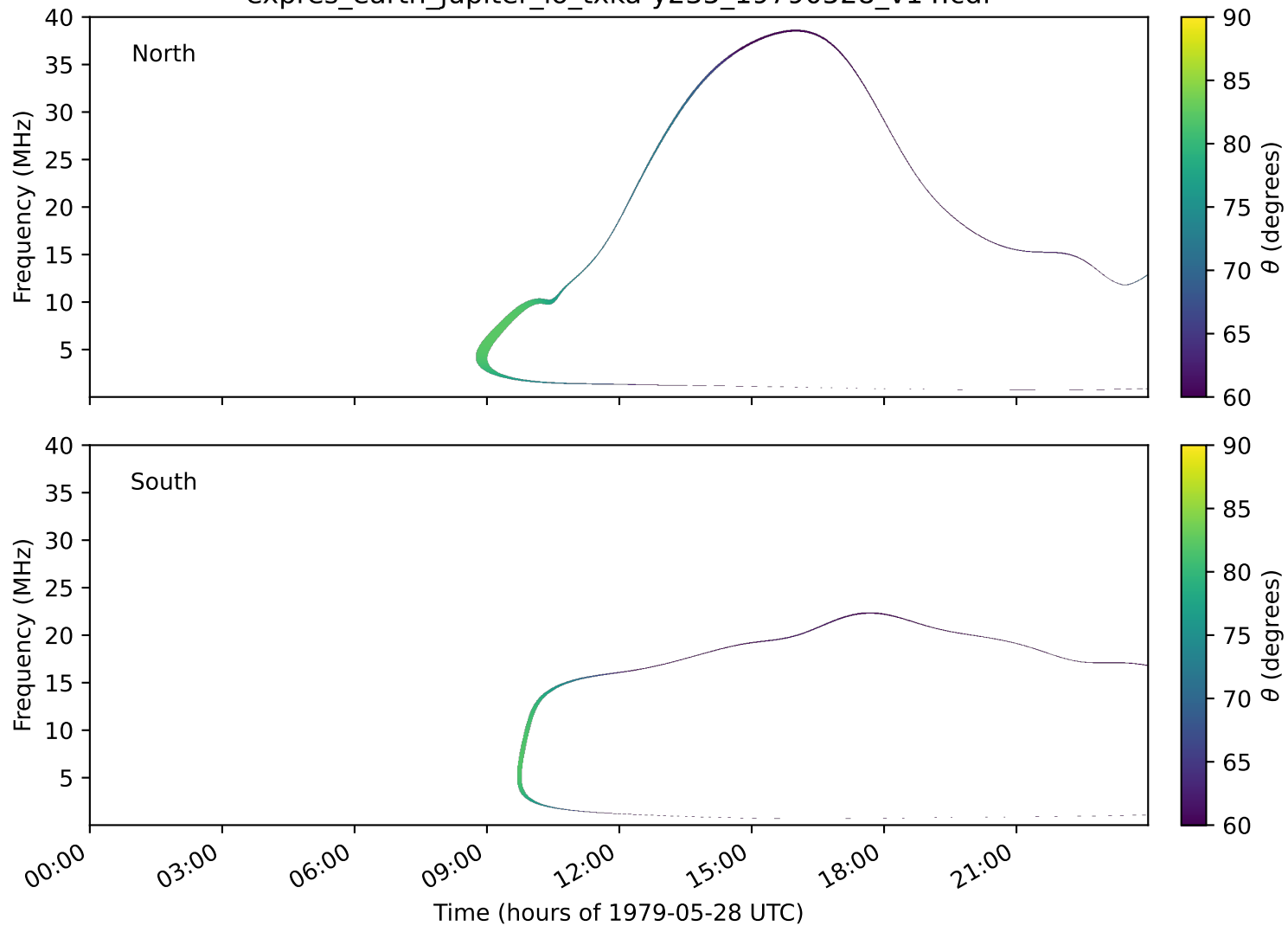
expres_earth_jupiter_io_txka-y235_19790528_v14.cdf
