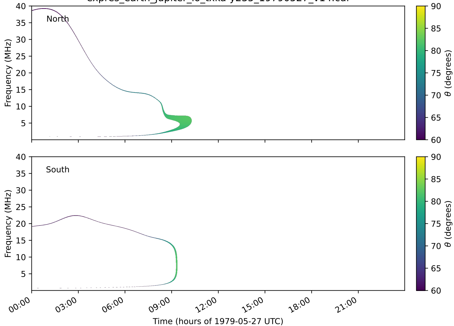
expres_earth_jupiter_io_txka-y235_19790527_v14.cdf
