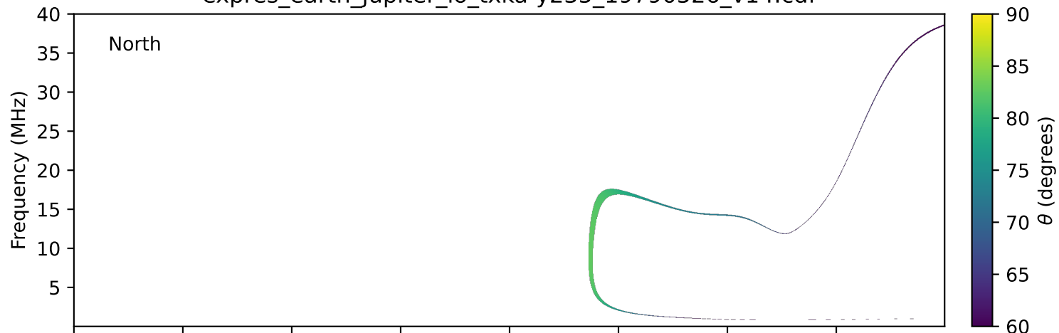
expres_earth_jupiter_io_txka-y235_19790526_v14.cdf
