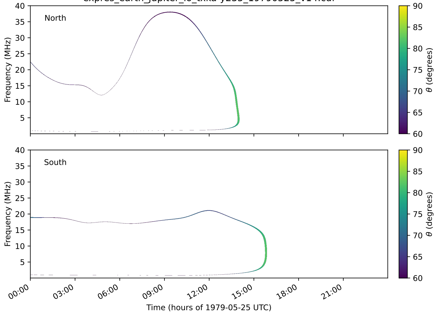
expres_earth_jupiter_io_txka-y235_19790525_v14.cdf
