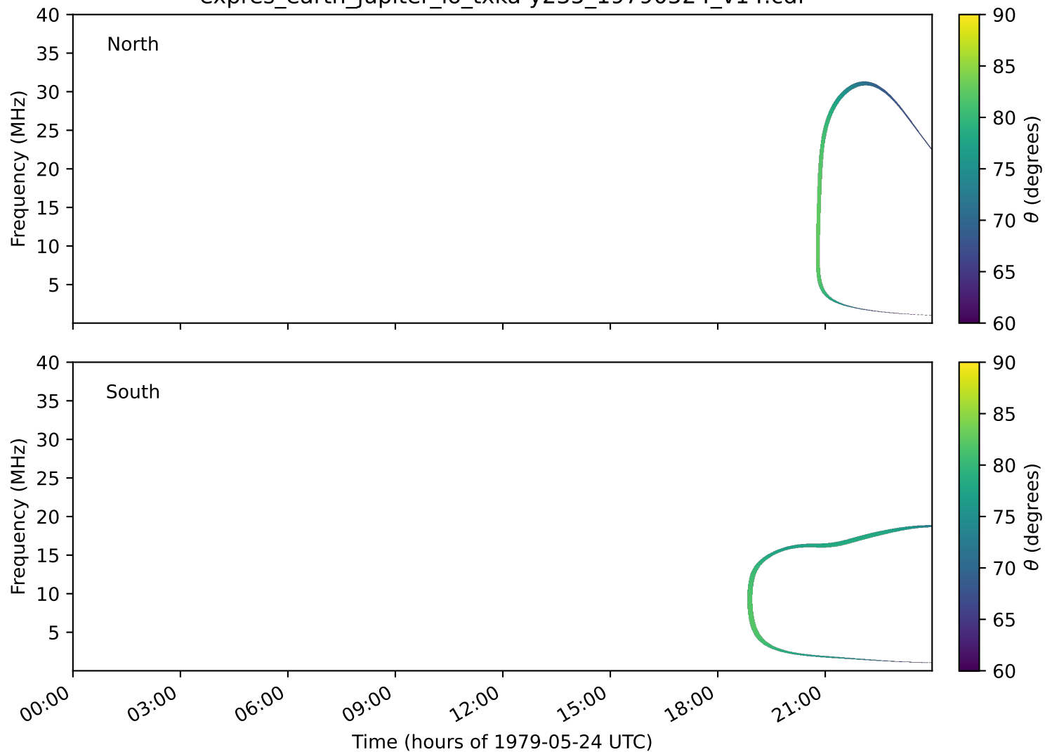
expres_earth_jupiter_io_txka-y235_19790524_v14.cdf
