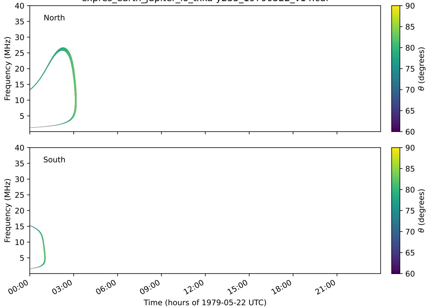
expres_earth_jupiter_io_txka-y235_19790522_v14.cdf
