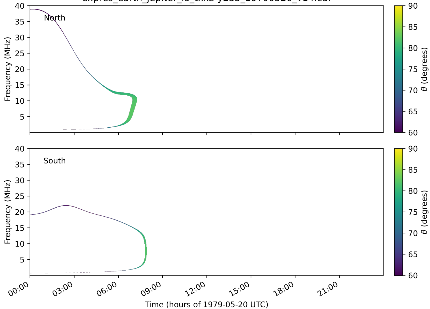
expres_earth_jupiter_io_txka-y235_19790520_v14.cdf
