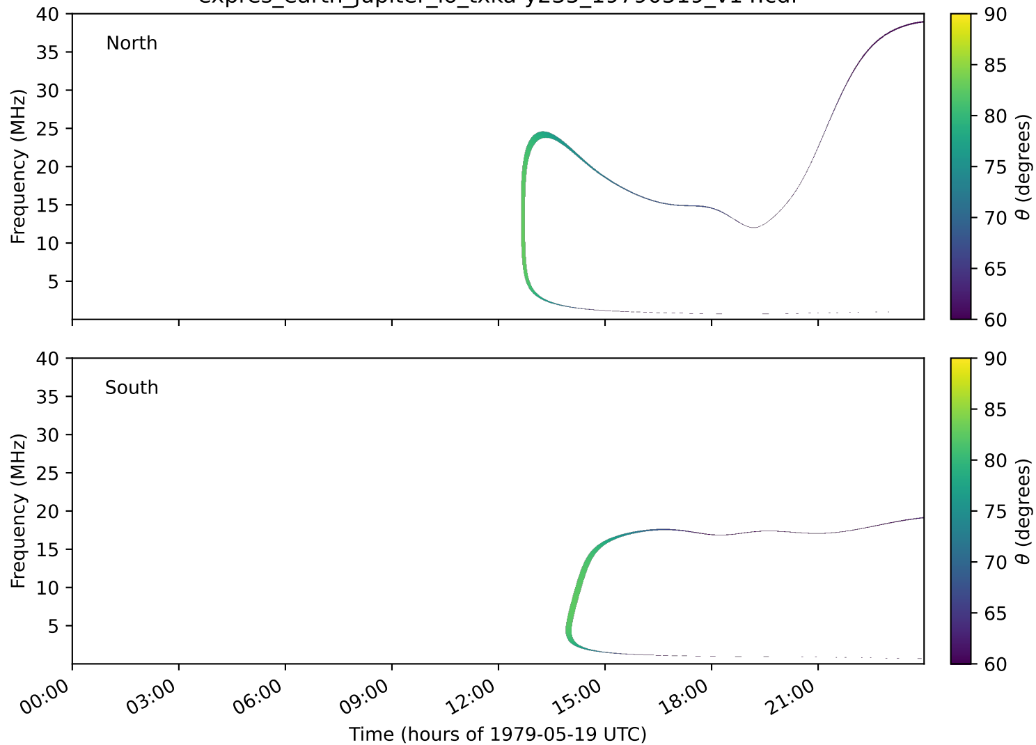
expres_earth_jupiter_io_txka-y235_19790519_v14.cdf
