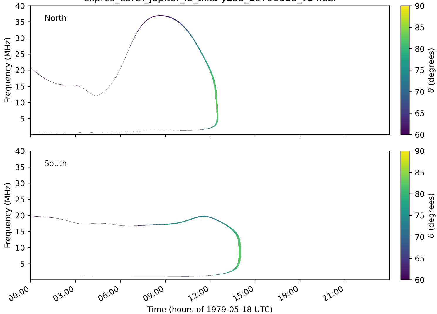
expres_earth_jupiter_io_txka-y235_19790518_v14.cdf
