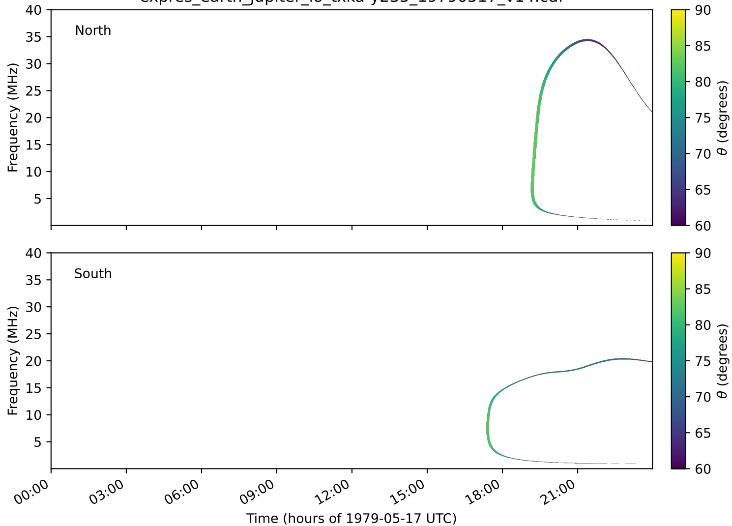
expres_earth_jupiter_io_txka-y235_19790517_v14.cdf
