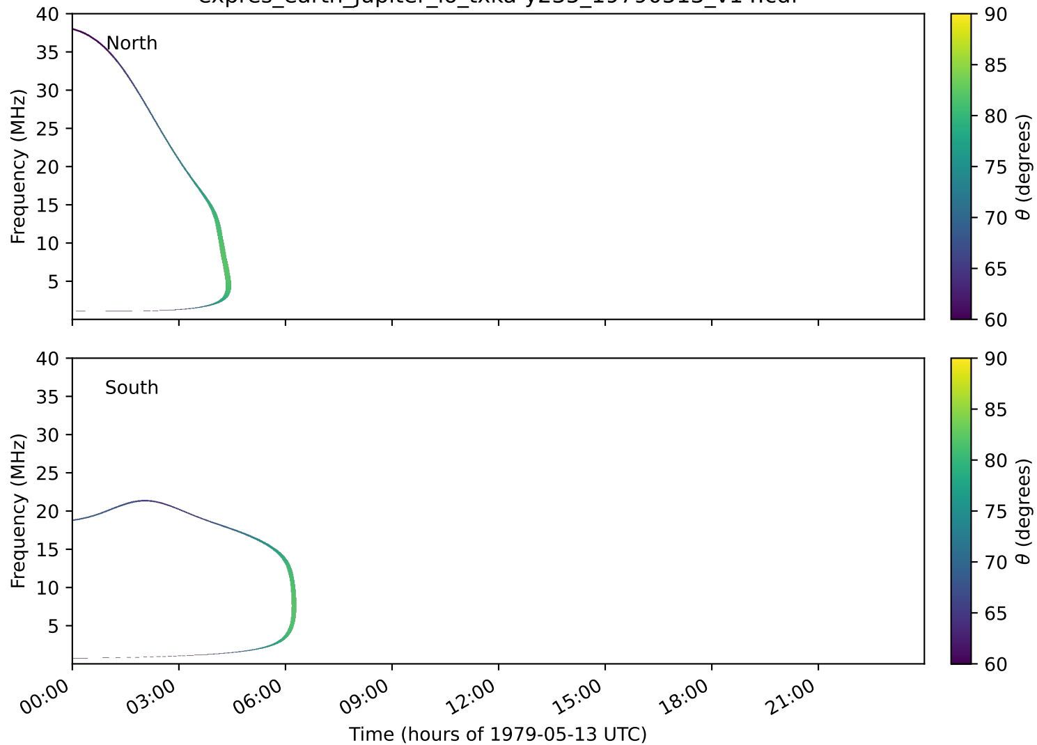
expres_earth_jupiter_io_txka-y235_19790513_v14.cdf
