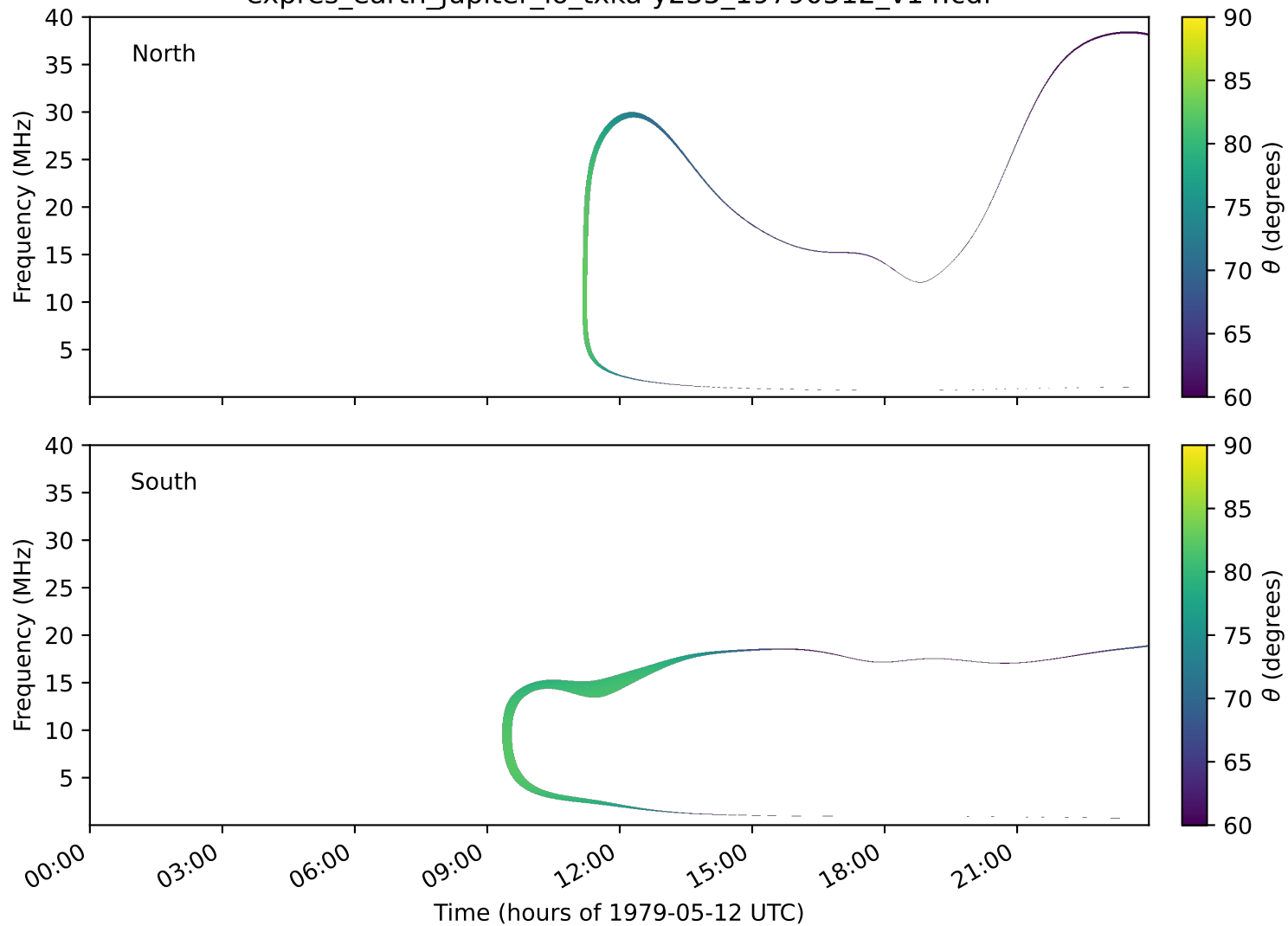
expres_earth_jupiter_io_txka-y235_19790512_v14.cdf
