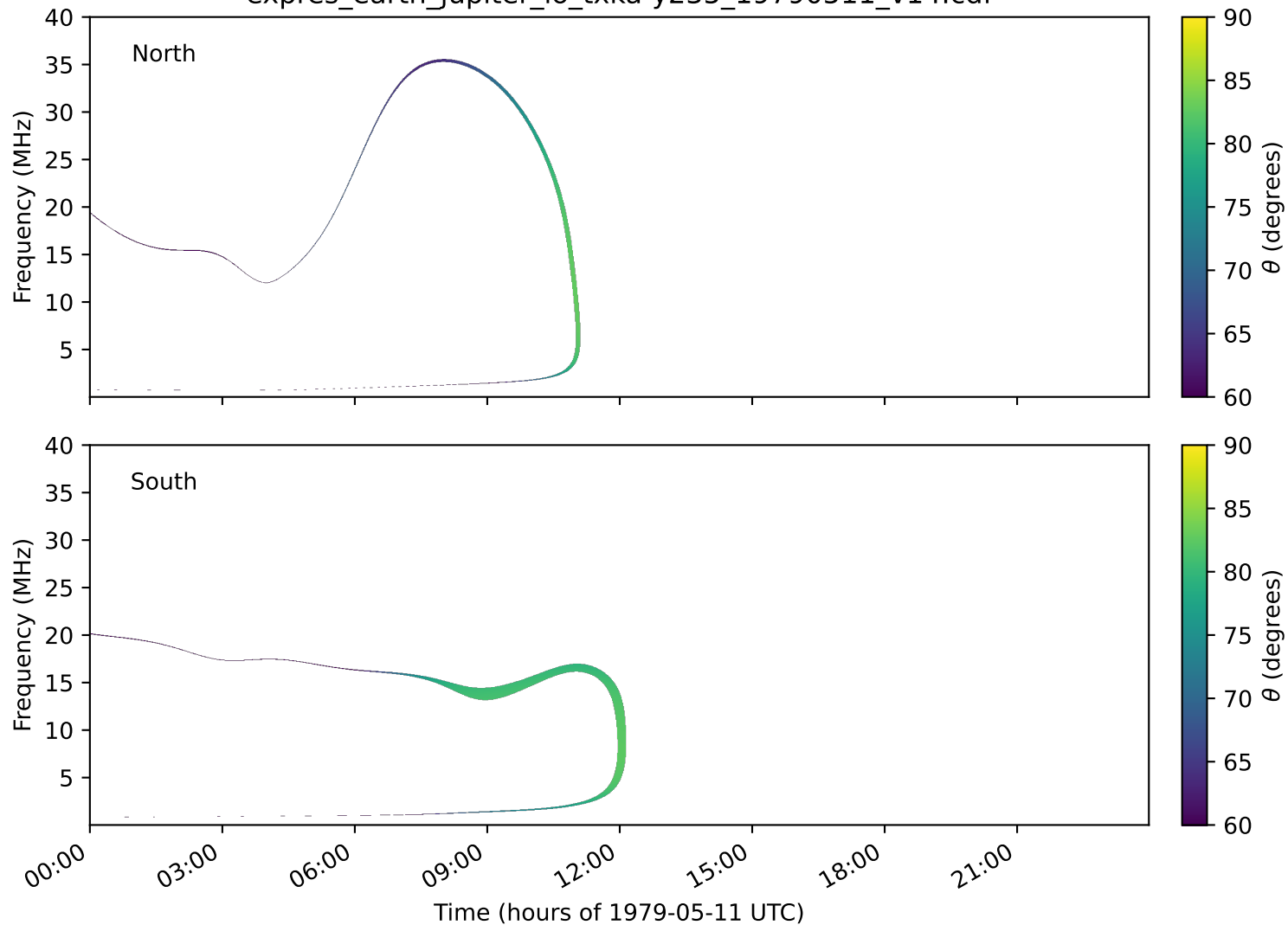
expres_earth_jupiter_io_txka-y235_19790511_v14.cdf
