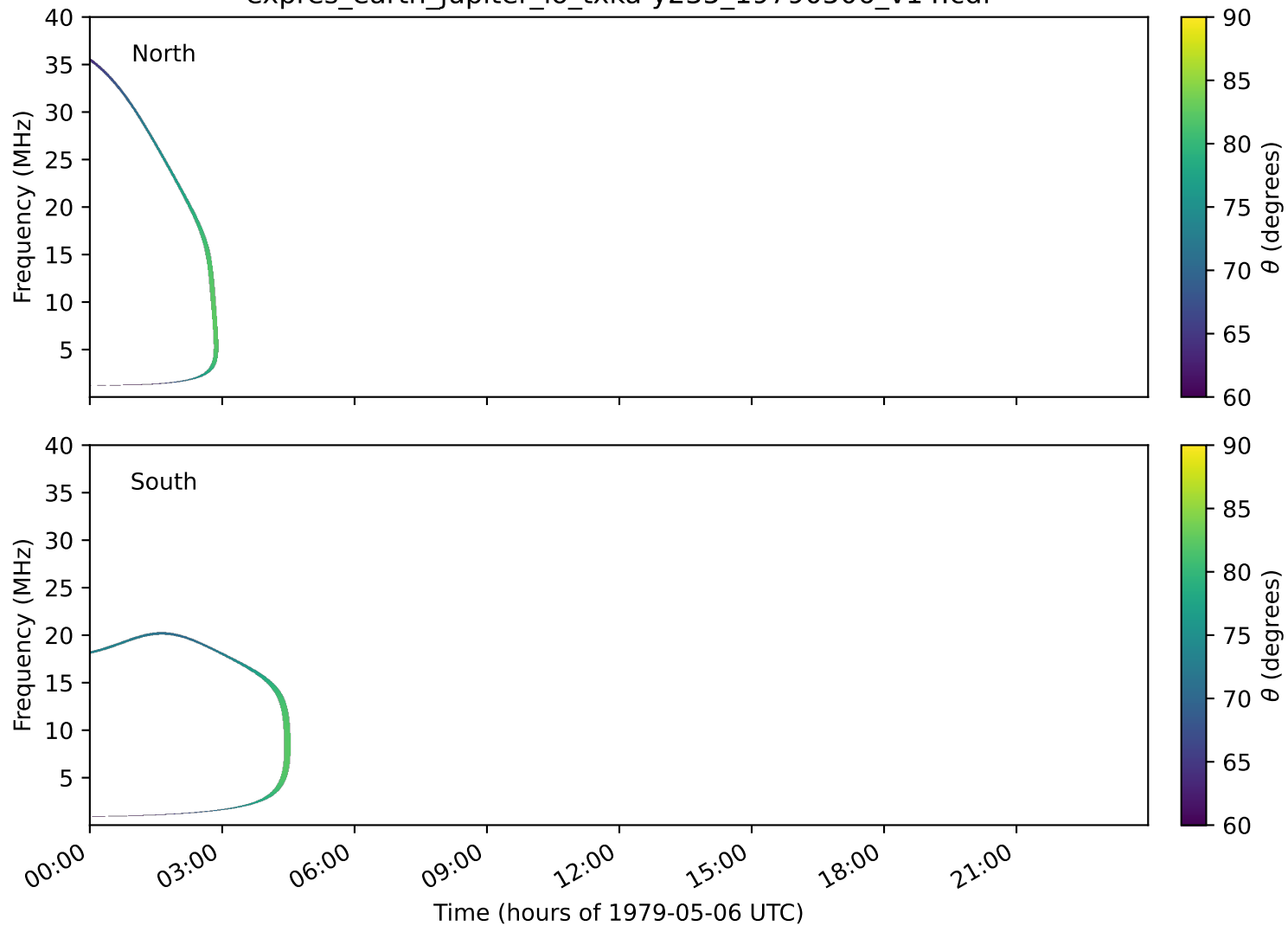
expres_earth_jupiter_io_txka-y235_19790506_v14.cdf
