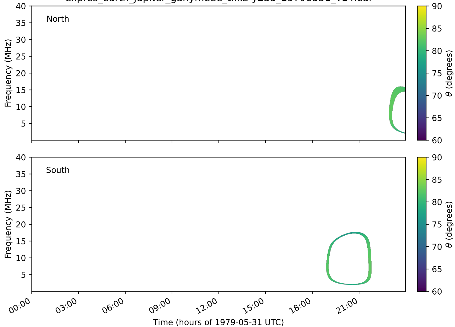
expres_earth_jupiter_ganymede_txka-y235_19790531_v14.cdf
