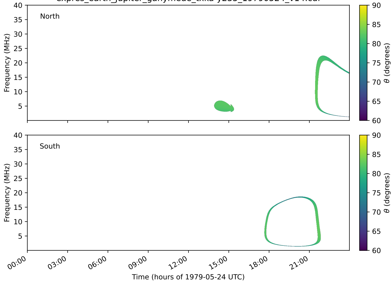
expres_earth_jupiter_ganymede_txka-y235_19790524_v14.cdf
