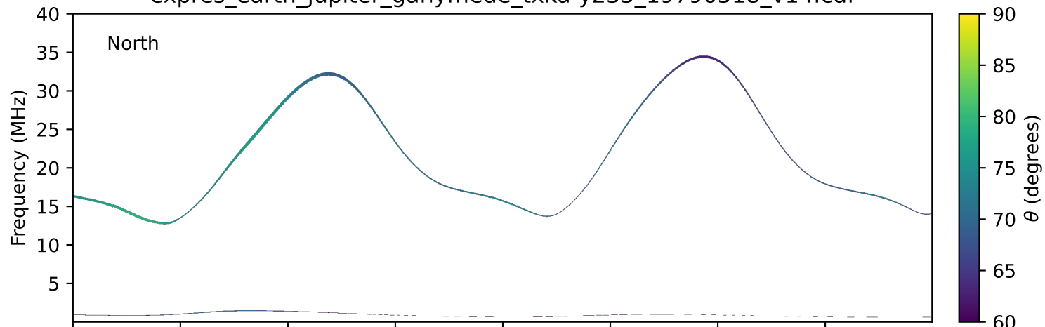
expres_earth_jupiter_ganymede_txka-y235_19790518_v14.cdf
