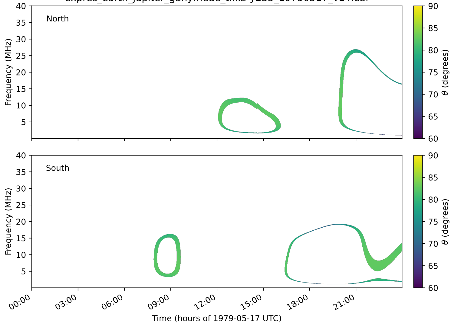
expres_earth_jupiter_ganymede_txka-y235_19790517_v14.cdf
