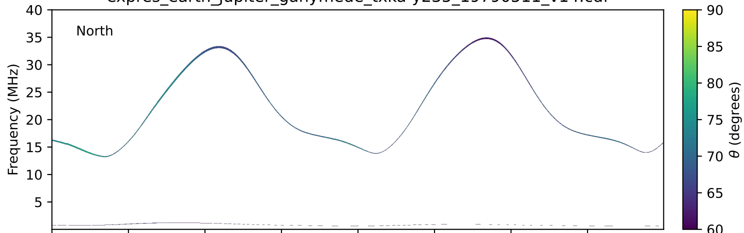
expres_earth_jupiter_ganymede_txka-y235_19790511_v14.cdf
