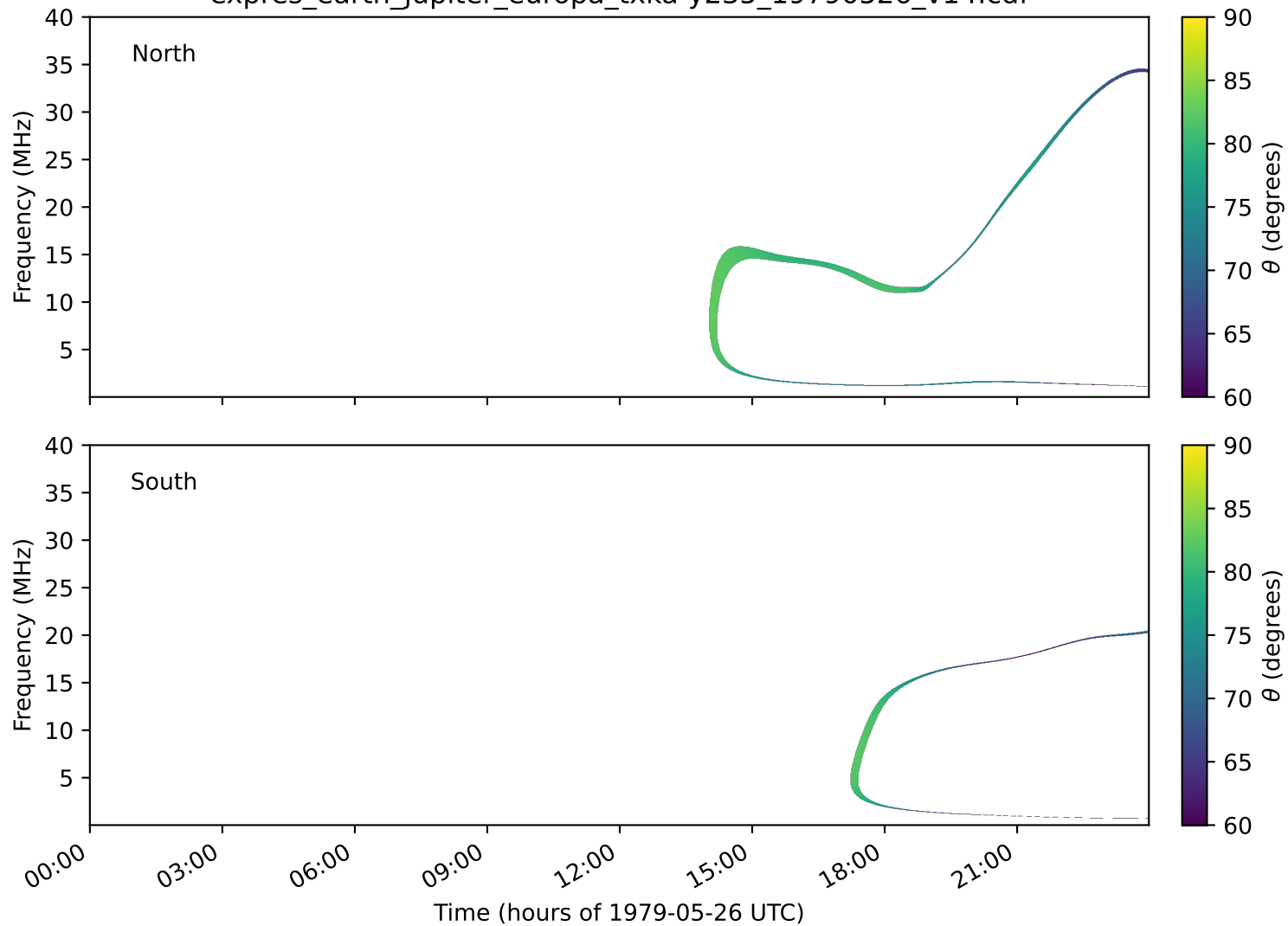
expres_earth_jupiter_europa_txka-y235_19790526_v14.cdf
