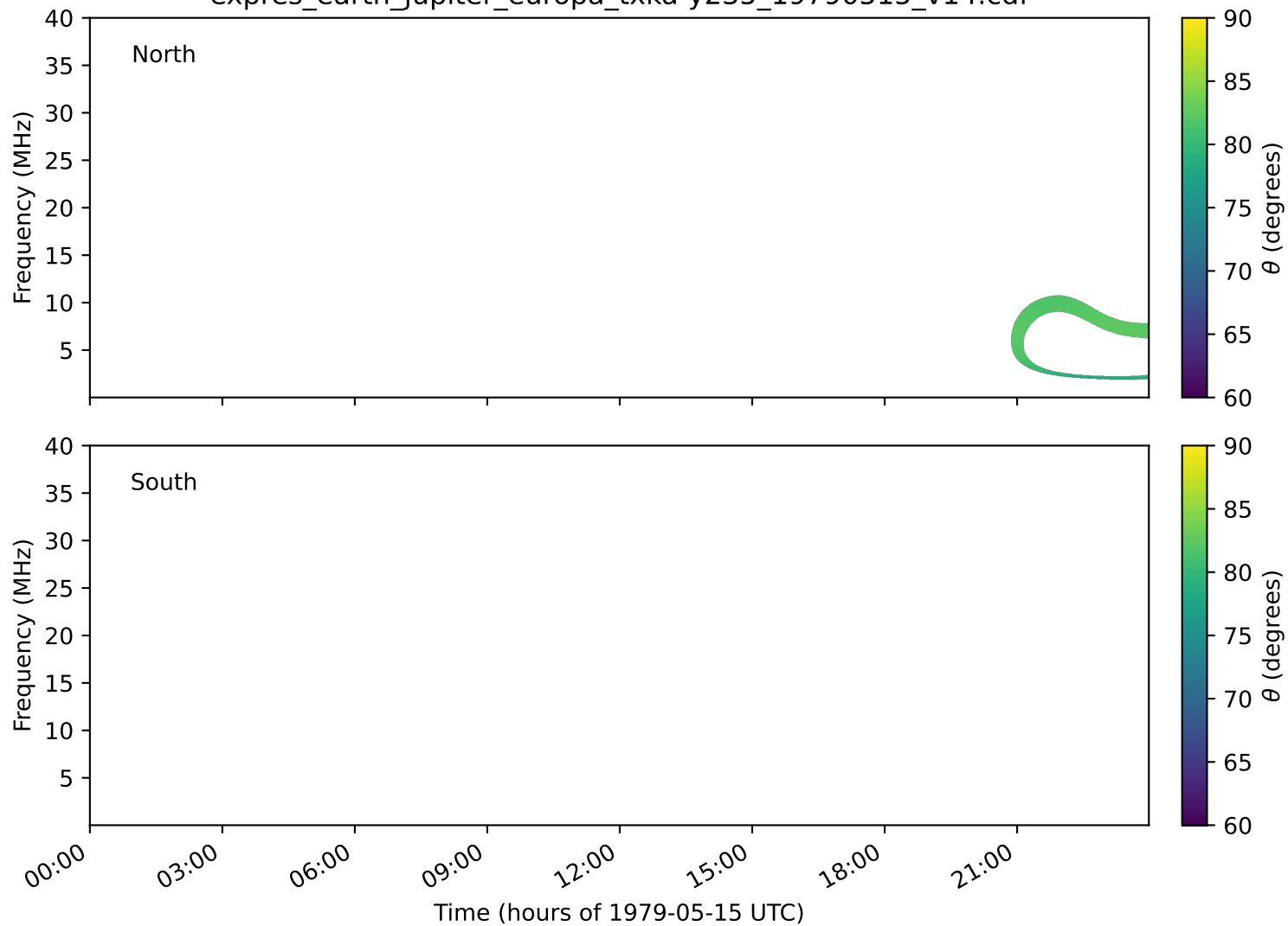
expres_earth_jupiter_europa_txka-y235_19790515_v14.cdf
