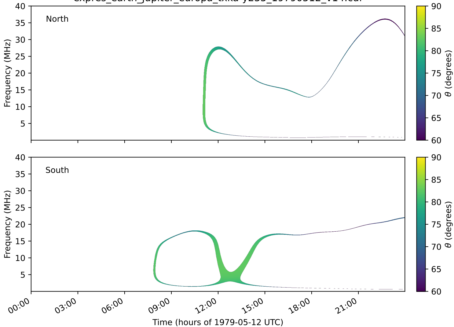
expres_earth_jupiter_europa_txka-y235_19790512_v14.cdf
