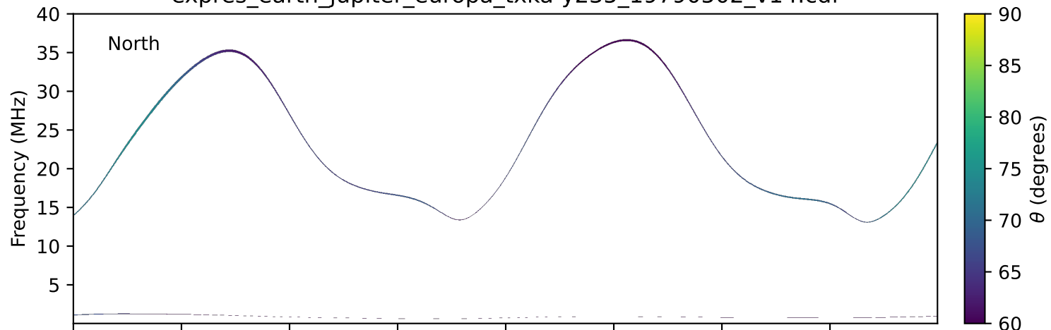
expres_earth_jupiter_europa_txka-y235_19790502_v14.cdf
