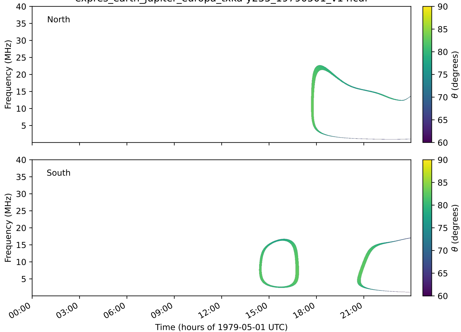
expres_earth_jupiter_europa_txka-y235_19790501_v14.cdf
